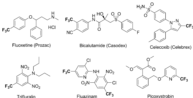
Scheme 1. Active ingredients of selected pharmaceuticals and agrochemicals containing a trifluoromethylated aromatic moiety.
