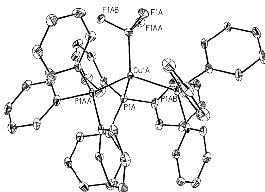
Figure 1. ORTEP drawing of one of the three molecules of 1 with thermal ellipsoids drawn at the 50 % probability level and all H atoms omitted for clarity.
